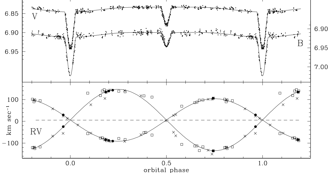
Fig. 1. Our photo-electric V (top) and B (bottom) observations of HD 23642 are phase plotted in the upper panel following the ephemeris of Table 2. The lower panel displays our radial velocities from Table 1 (filled circles) and those from Pearce (1957, squares) and Abt (1958, crosses). The curves over plot the orbital solution given in Table 2.
